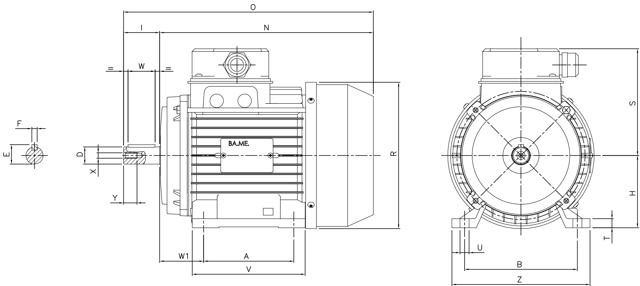
FORMA B3 – DIMENSIONI / FRAME SIZE B3 FORM
